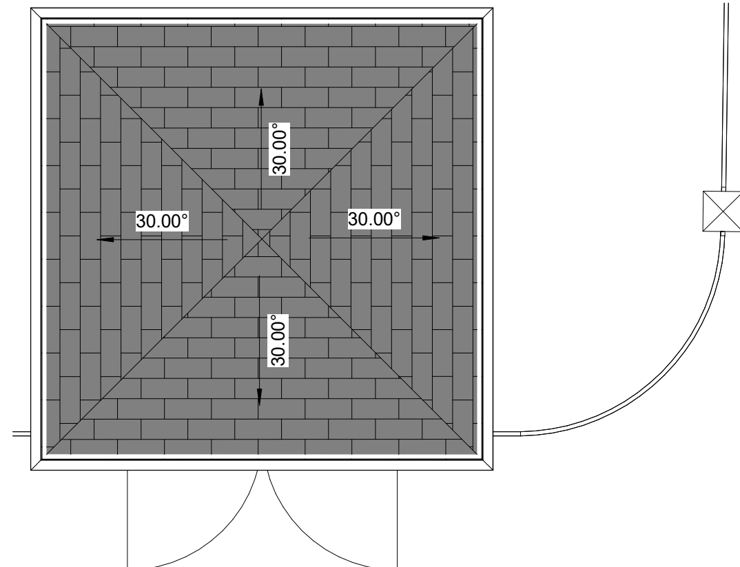
Sub Station Roof Plan
