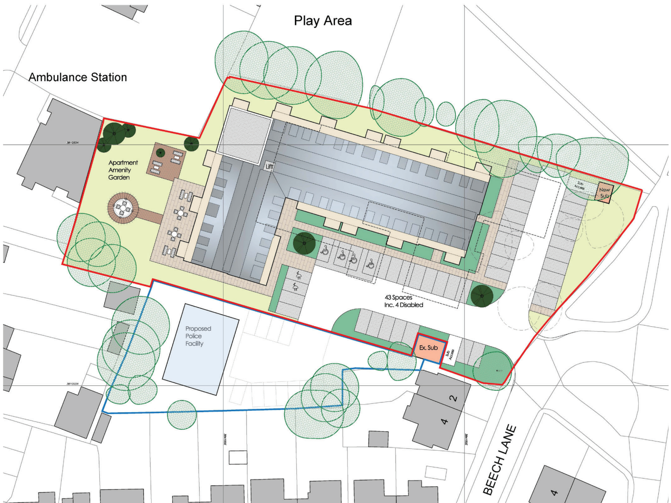
Proposed site layout of McCarthy Stone's proposals for land at Wilmslow Police Station, Beech Lane, Wilmslow
